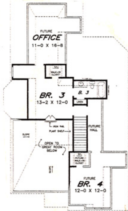
Second Floor Plan (A)
